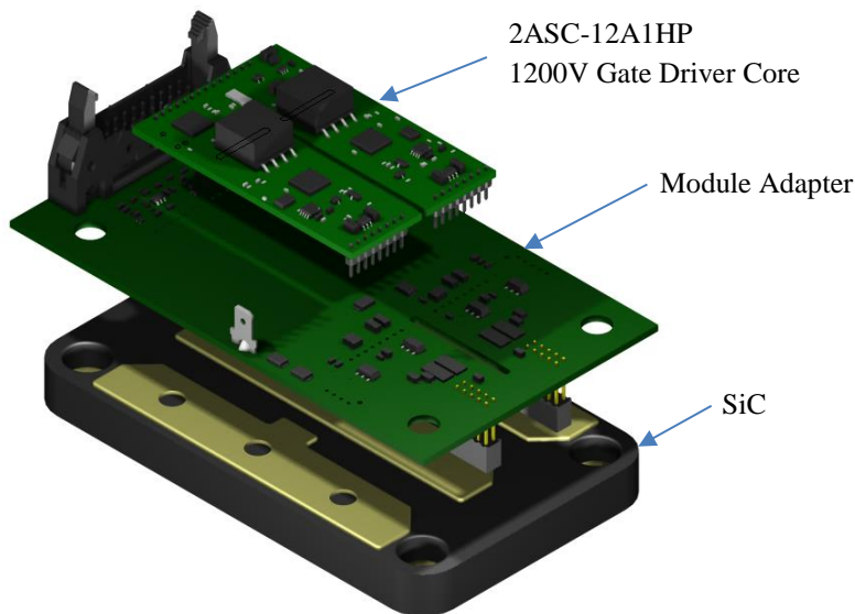
High Performance 62mm Half-Bridge Module Adapter for 2ASC-12A1HP
