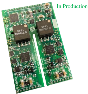
2ASC-12A1HP 1200V Dual-Channel Core 3W/10A
